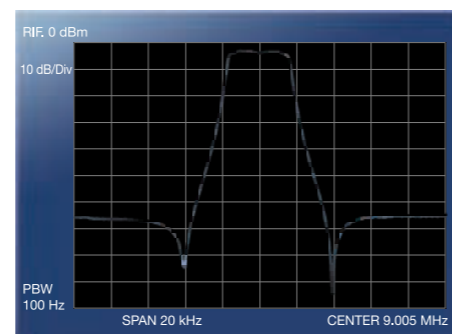
Filtro roofing 3 kHz (9 MHz, SPAN: 20 kHz)
