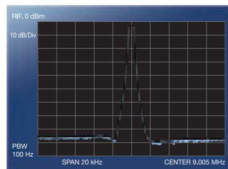
Filtro roofing 600 Hz (9 MHz, SPAN: 20 kHz)
