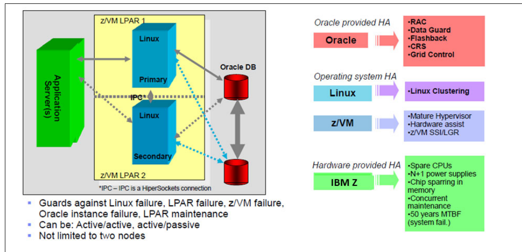
Figure 6-1 Building blocks of an HA environment for Oracle Database on Linux running on LinuxONE
