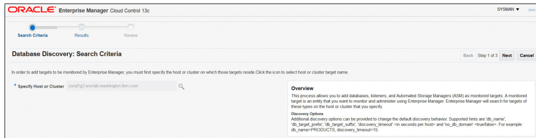
Figure 3-19 Selecting target
