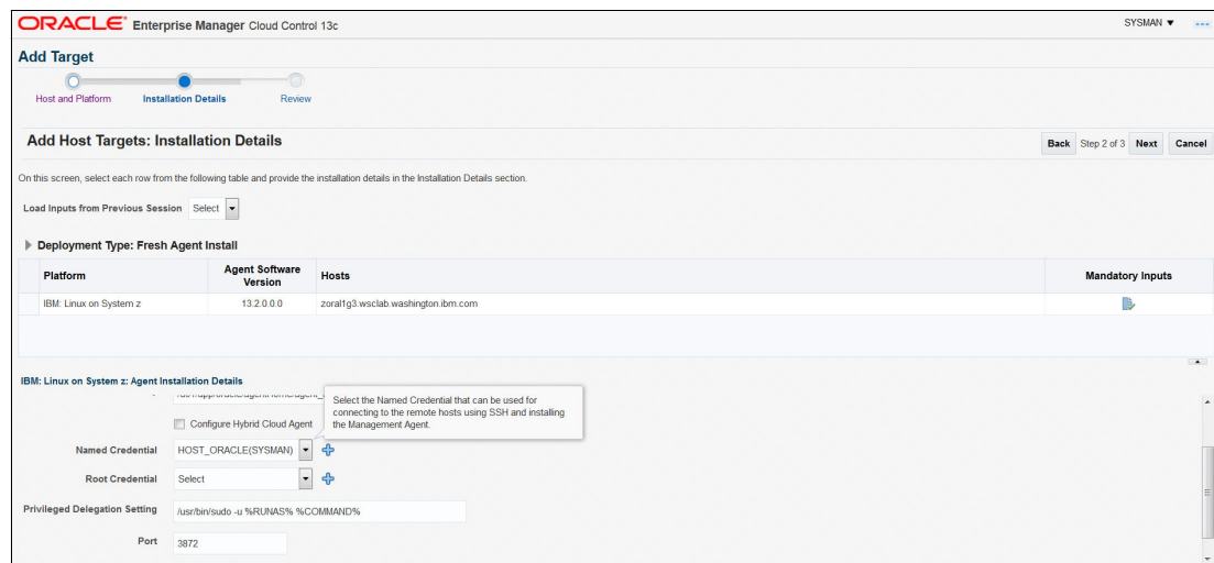
Figure 3-13 Installation information
