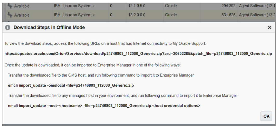
Figure 3-11 Offline download
